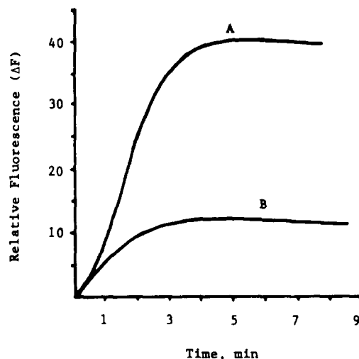
Fig. 9. Fluorescence change ( \Delta F ) as a function of time upon addition of 0.25 \mu\text{g/ml} phospholipase A_2 to solutions containing 1 \times 10^{-5} M DPPC, 5 \times 10^{-5} M ANS, 6 \times 10^{-3} M \text{Ca}^{2+} , and in the absence (A) and presence of 6 \times 10^{-3} M chlorphentermine (B). Drug inhibition of enzyme activities is indicated by the reduction of fluorescence enhancement.
