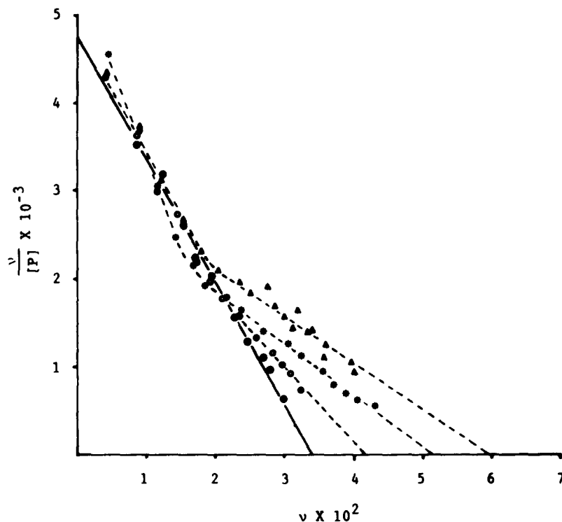
Fig. 8. Effect of dopamine (●), phenylpropanolamine (○), ephedrine (*), and phentermine (△) on the binding of ANS to DPPC. Data were obtained from solutions containing 2 \times 10^{-5} M DPPC, 10^{-2} M drug, and varying concentrations of ANS and treated using equation 1.
